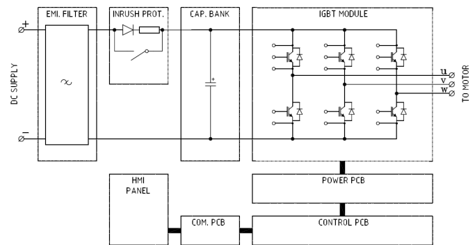
Block diagram for the DC/AC-converter.
